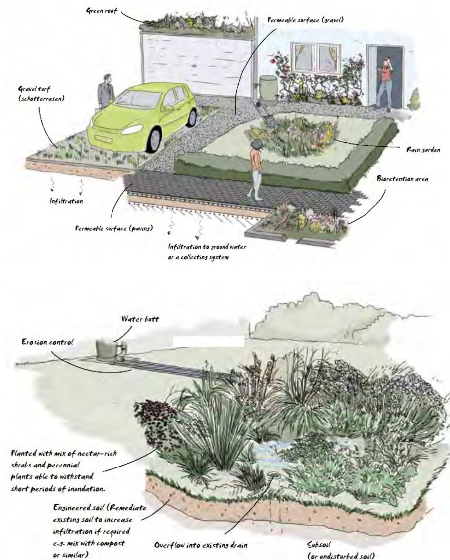
Figure 18- Example SuDS sketches of various permeable surfaces and rain garden attenuate (Source: RSPB 20 )
